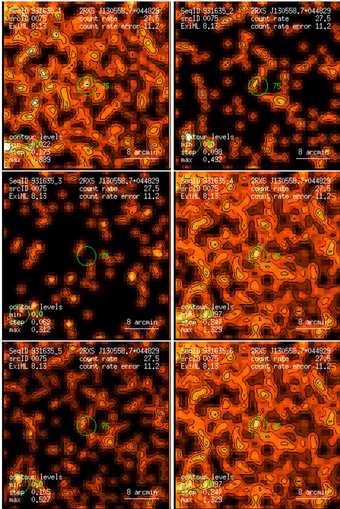
Figure 75: RASS 931635: detection 0075: band rate images, Gaussian filter: (1) PSPC channels 11 – 41, (2) 52 – 90, (3) 91 – 201, (4) 11 – 235, (5) 52 – 201, (6) 11 – 201. Broad band rates in counts/ks. Band rate contour levels in counts/ks/arcmin 2 .
