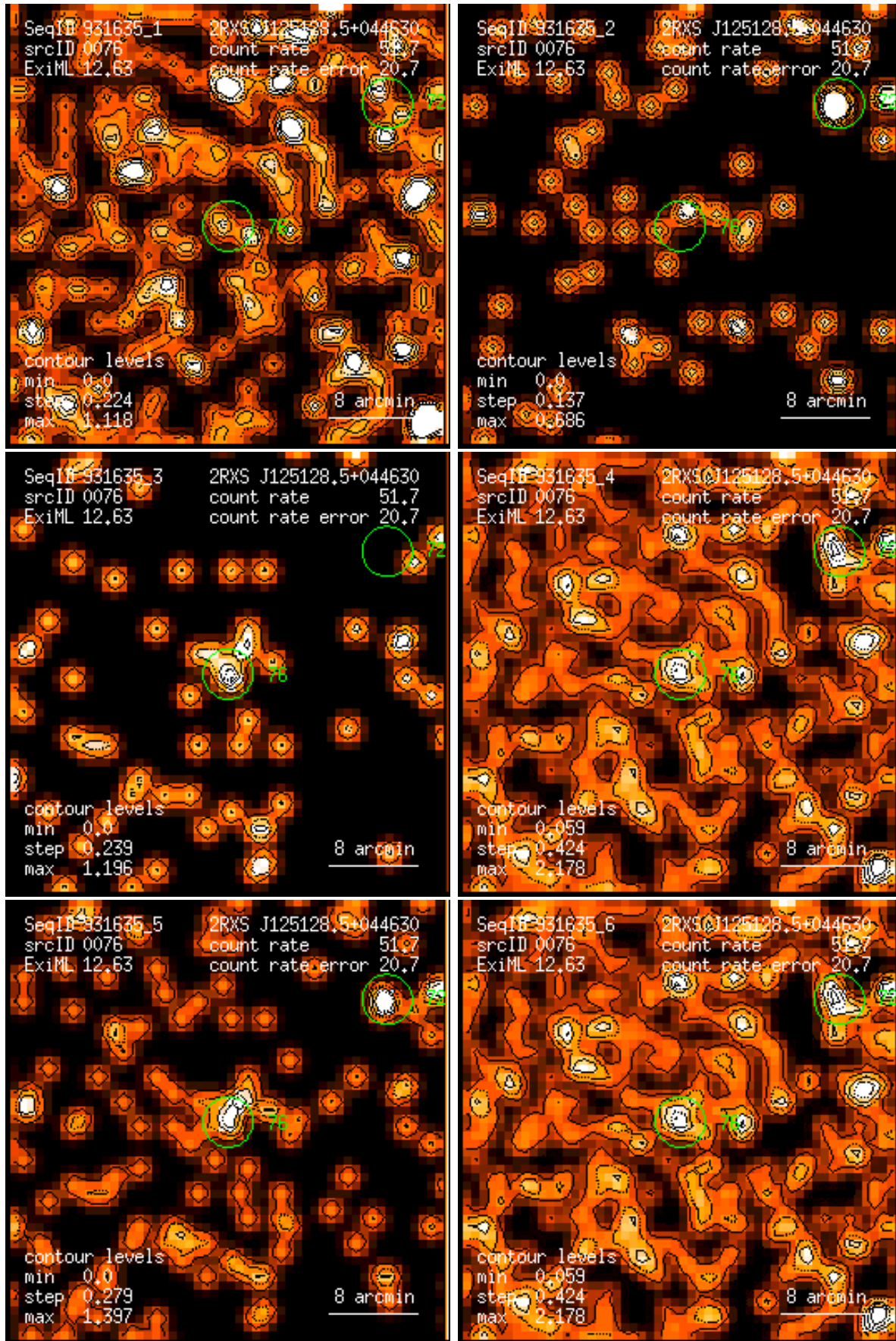
Figure 76: RASS 931635: detection 0076: band rate images, Gaussian filter: (1) PSPC channels 11 – 41, (2) 52 – 90, (3) 91 – 201, (4) 11 – 235, (5) 52 – 201, (6) 11 – 201. Broad band rates in counts/ks. Band rate contour levels in counts/ks/arcmin 2 .
