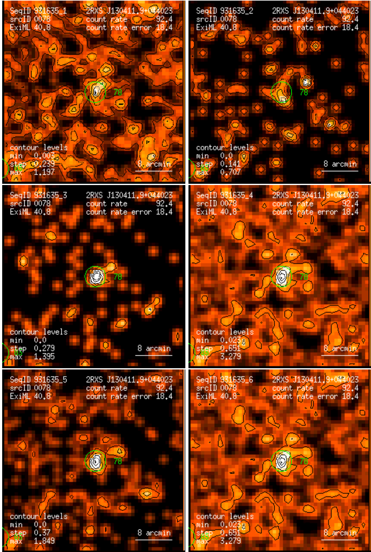
Figure 78: RASS 931635: detection 0078: band rate images, Gaussian filter: (1) PSPC channels 11 – 41, (2) 52 – 90, (3) 91 – 201, (4) 11 – 235, (5) 52 – 201, (6) 11 – 201. Broad band rates in counts/ks. Band rate contour levels in counts/ks/arcmin 2 .
