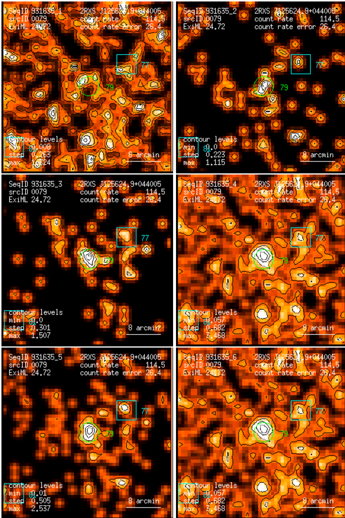
Figure 79: RASS 931635: detection 0079: band rate images, Gaussian filter: (1) PSPC channels 11 – 41, (2) 52 – 90, (3) 91 – 201, (4) 11 – 235, (5) 52 – 201, (6) 11 – 201. Broad band rates in counts/ks. Band rate contour levels in counts/ks/arcmin 2 .
