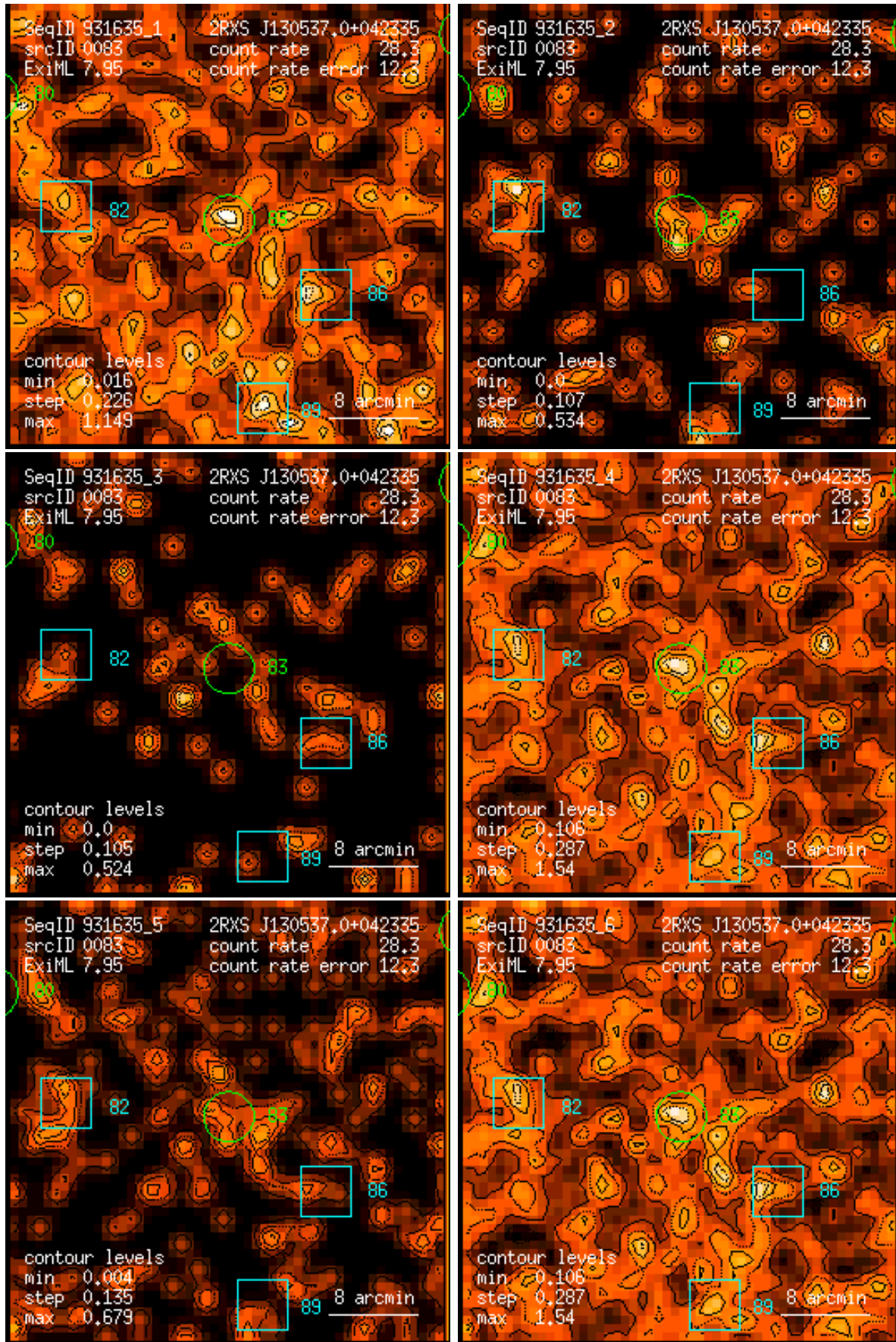
Figure 83: RASS 931635: detection 0083: band rate images, Gaussian filter: (1) PSPC channels 11 – 41, (2) 52 – 90, (3) 91 – 201, (4) 11 – 235, (5) 52 – 201, (6) 11 – 201. Broad band rates in counts/ks. Band rate contour levels in counts/ks/arcmin 2 .
