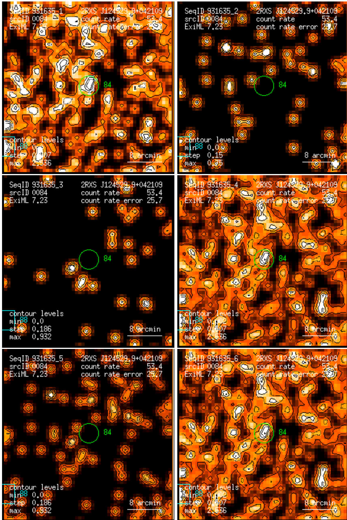
Figure 84: RASS 931635: detection 0084: band rate images, Gaussian filter: (1) PSPC channels 11 – 41, (2) 52 – 90, (3) 91 – 201, (4) 11 – 235, (5) 52 – 201, (6) 11 – 201. Broad band rates in counts/ks. Band rate contour levels in counts/ks/arcmin 2 .
