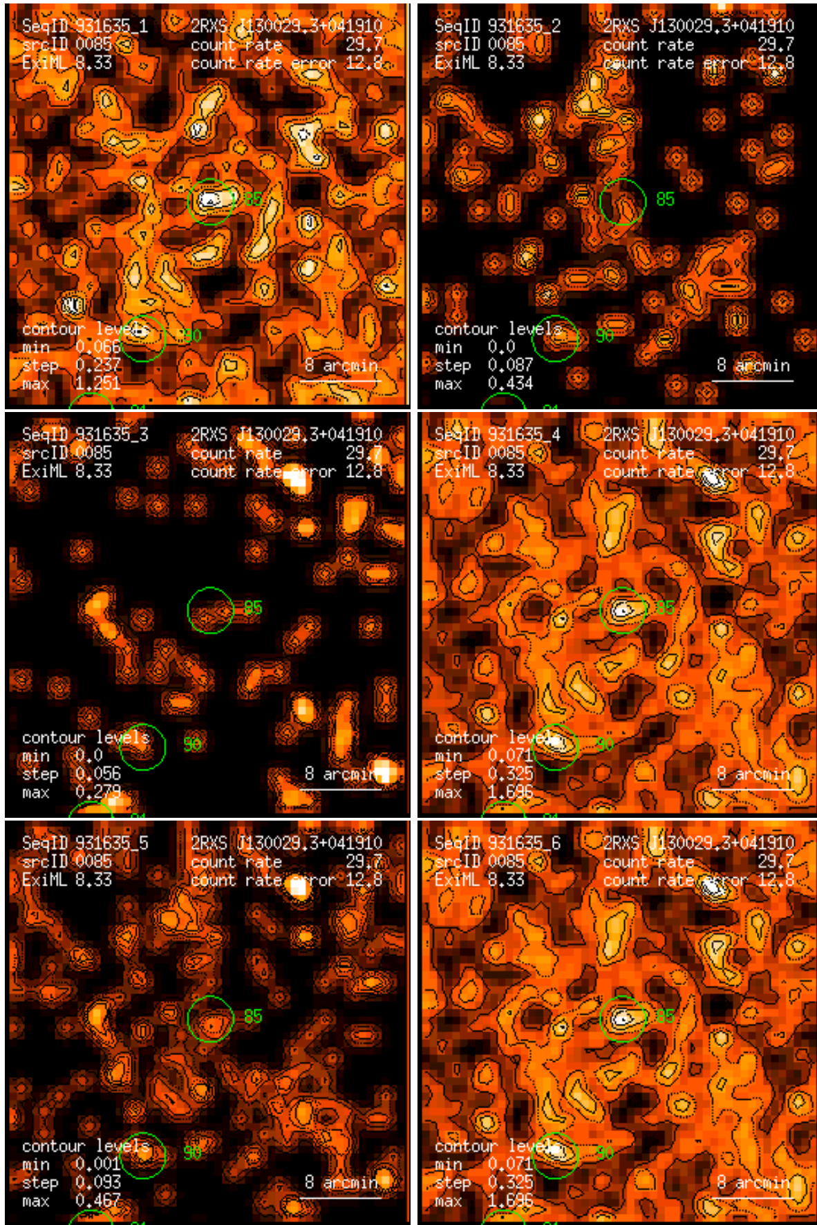
Figure 85: RASS 931635: detection 0085: band rate images, Gaussian filter: (1) PSPC channels 11 – 41, (2) 52 – 90, (3) 91 – 201, (4) 11 – 235, (5) 52 – 201, (6) 11 – 201. Broad band rates in counts/ks. Band rate contour levels in counts/ks/arcmin 2 .
