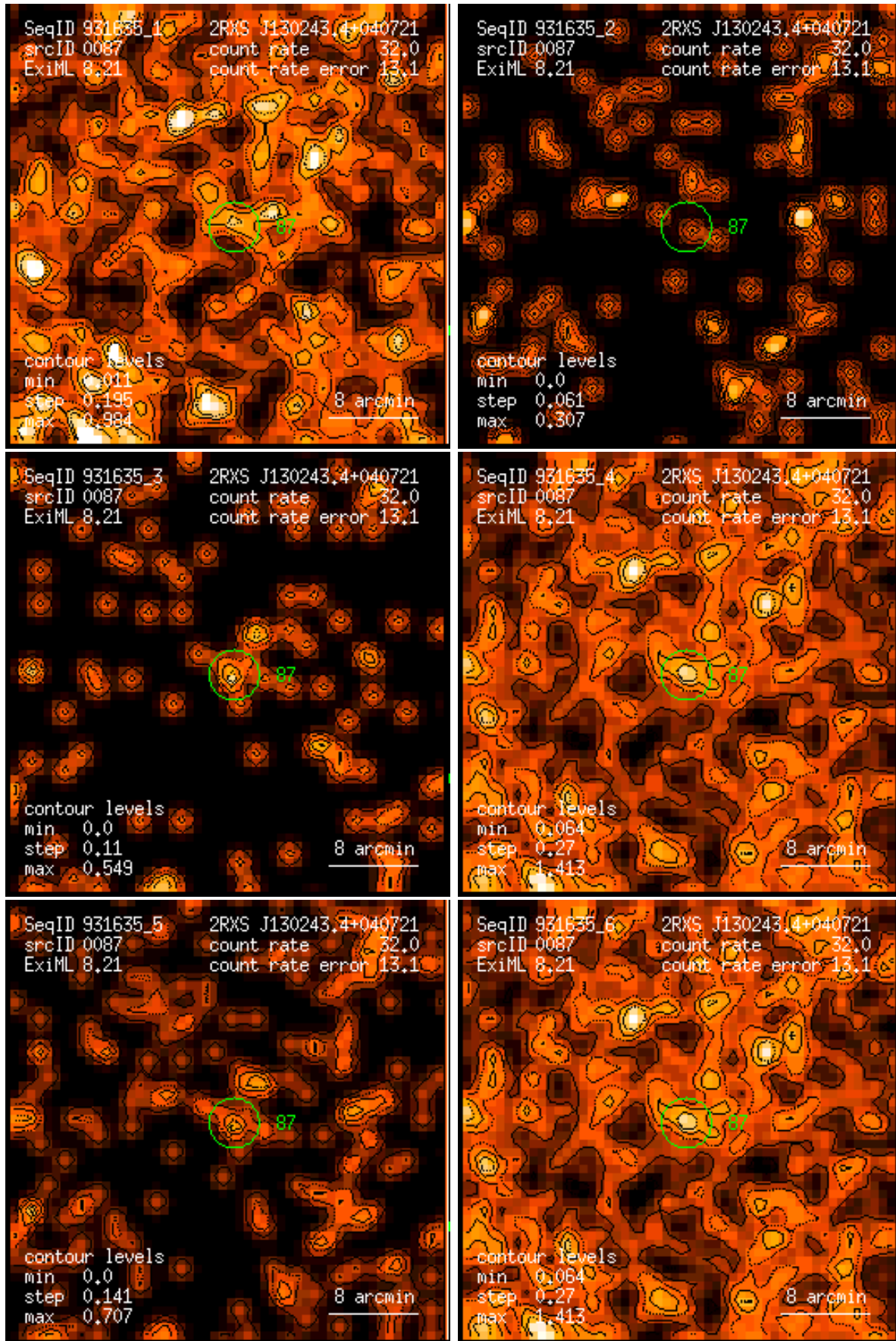
Figure 87: RASS 931635: detection 0087: band rate images, Gaussian filter: (1) PSPC channels 11 – 41, (2) 52 – 90, (3) 91 – 201, (4) 11 – 235, (5) 52 – 201, (6) 11 – 201. Broad band rates in counts/ks. Band rate contour levels in counts/ks/arcmin 2 .
