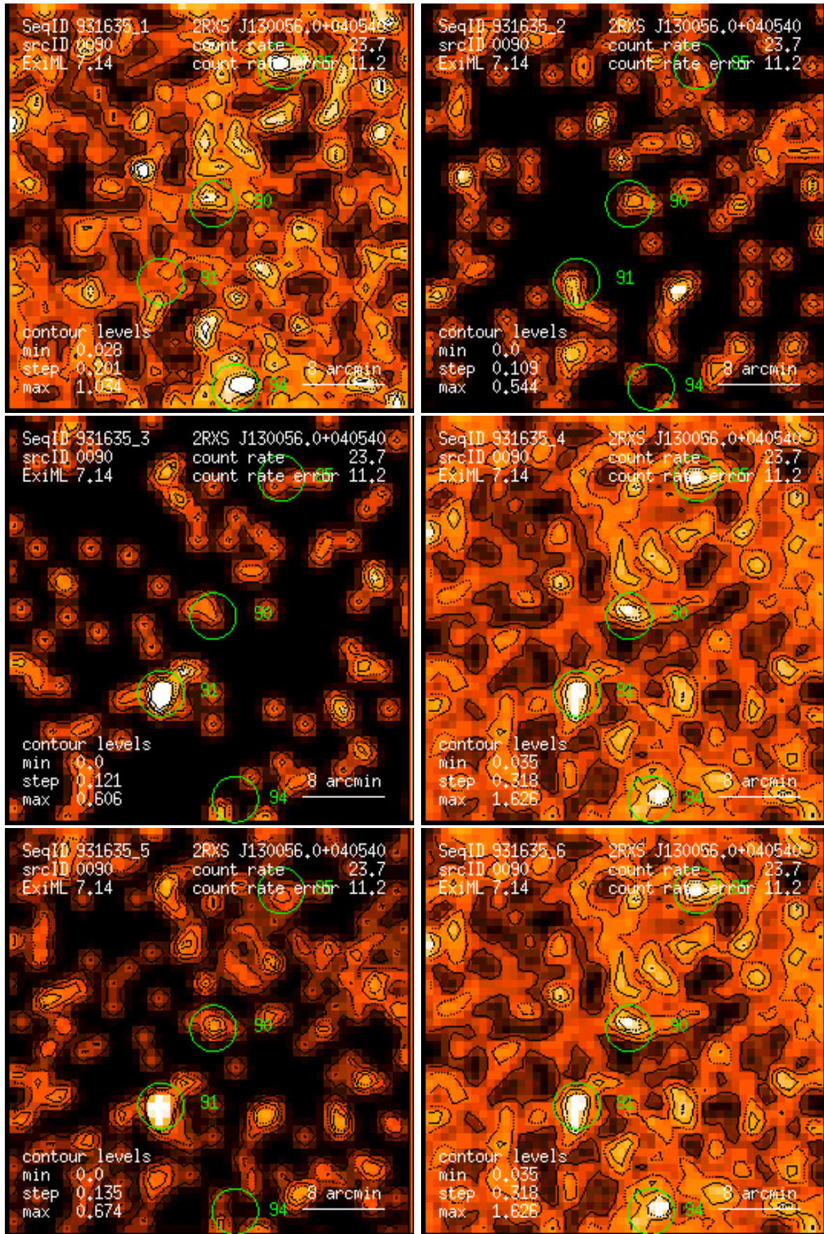
Figure 90: RASS 931635: detection 0090: band rate images, Gaussian filter: (1) PSPC channels 11 – 41, (2) 52 – 90, (3) 91 – 201, (4) 11 – 235, (5) 52 – 201, (6) 11 – 201. Broad band rates in counts/ks. Band rate contour levels in counts/ks/arcmin 2 .
