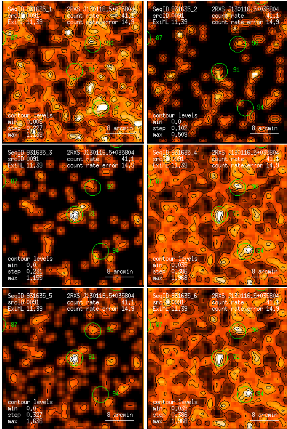
Figure 91: RASS 931635: detection 0091: band rate images, Gaussian filter: (1) PSPC channels 11 – 41, (2) 52 – 90, (3) 91 – 201, (4) 11 – 235, (5) 52 – 201, (6) 11 – 201. Broad band rates in counts/ks. Band rate contour levels in counts/ks/arcmin 2 .
