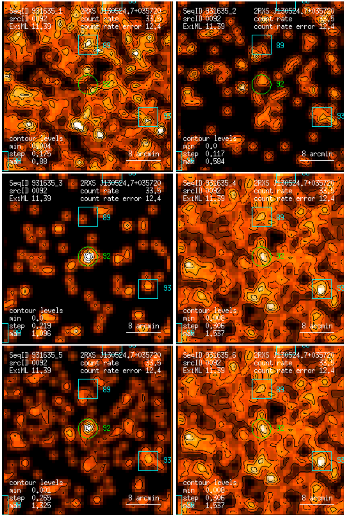
Figure 92: RASS 931635: detection 0092: band rate images, Gaussian filter: (1) PSPC channels 11 – 41, (2) 52 – 90, (3) 91 – 201, (4) 11 – 235, (5) 52 – 201, (6) 11 – 201. Broad band rates in counts/ks. Band rate contour levels in counts/ks/arcmin 2 .
