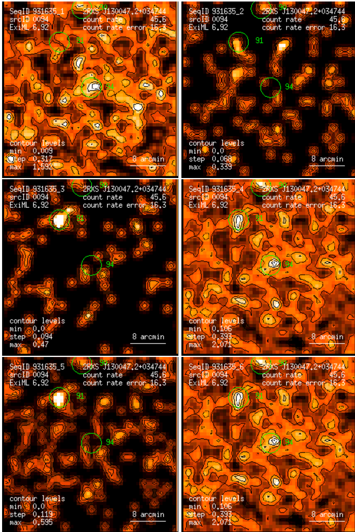
Figure 94: RASS 931635: detection 0094: band rate images, Gaussian filter: (1) PSPC channels 11 – 41, (2) 52 – 90, (3) 91 – 201, (4) 11 – 235, (5) 52 – 201, (6) 11 – 201. Broad band rates in counts/ks. Band rate contour levels in counts/ks/arcmin 2 .
