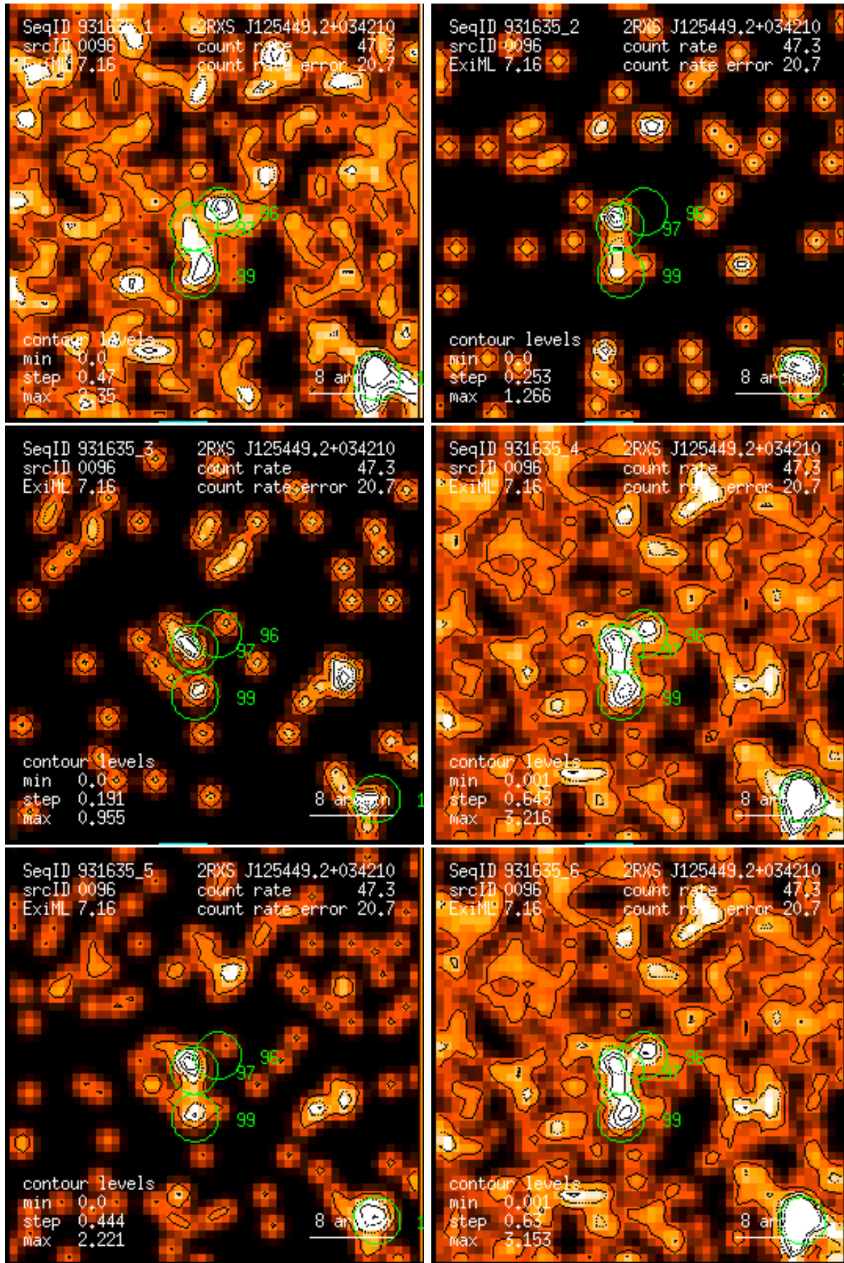
Figure 96: RASS 931635: detection 0096: band rate images, Gaussian filter: (1) PSPC channels 11 – 41, (2) 52 – 90, (3) 91 – 201, (4) 11 – 235, (5) 52 – 201, (6) 11 – 201. Broad band rates in counts/ks. Band rate contour levels in counts/ks/arcmin 2 .
