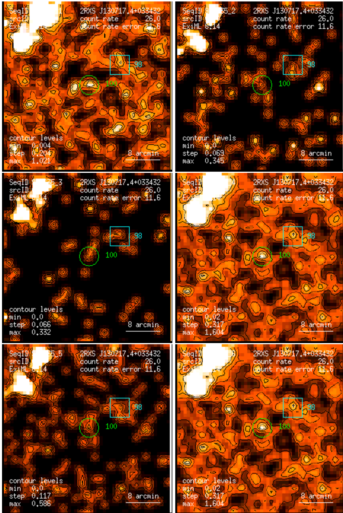
Figure 100: RASS 931635: detection 0100: band rate images, Gaussian filter: (1) PSPC channels 11 – 41, (2) 52 – 90, (3) 91 – 201, (4) 11 – 235, (5) 52 – 201, (6) 11 – 201. Broad band rates in counts/ks. Band rate contour levels in counts/ks/arcmin 2 .
