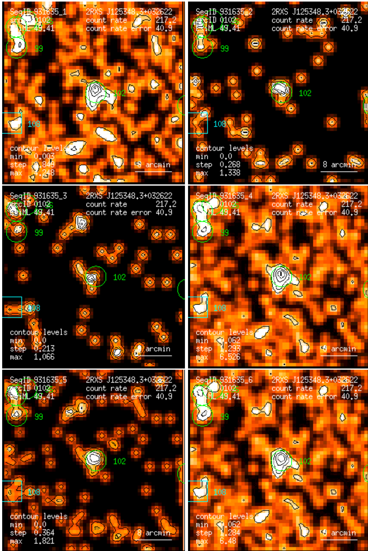
Figure 102: RASS 931635: detection 0102: band rate images, Gaussian filter: (1) PSPC channels 11 – 41, (2) 52 – 90, (3) 91 – 201, (4) 11 – 235, (5) 52 – 201, (6) 11 – 201. Broad band rates in counts/ks. Band rate contour levels in counts/ks/arcmin 2 .
