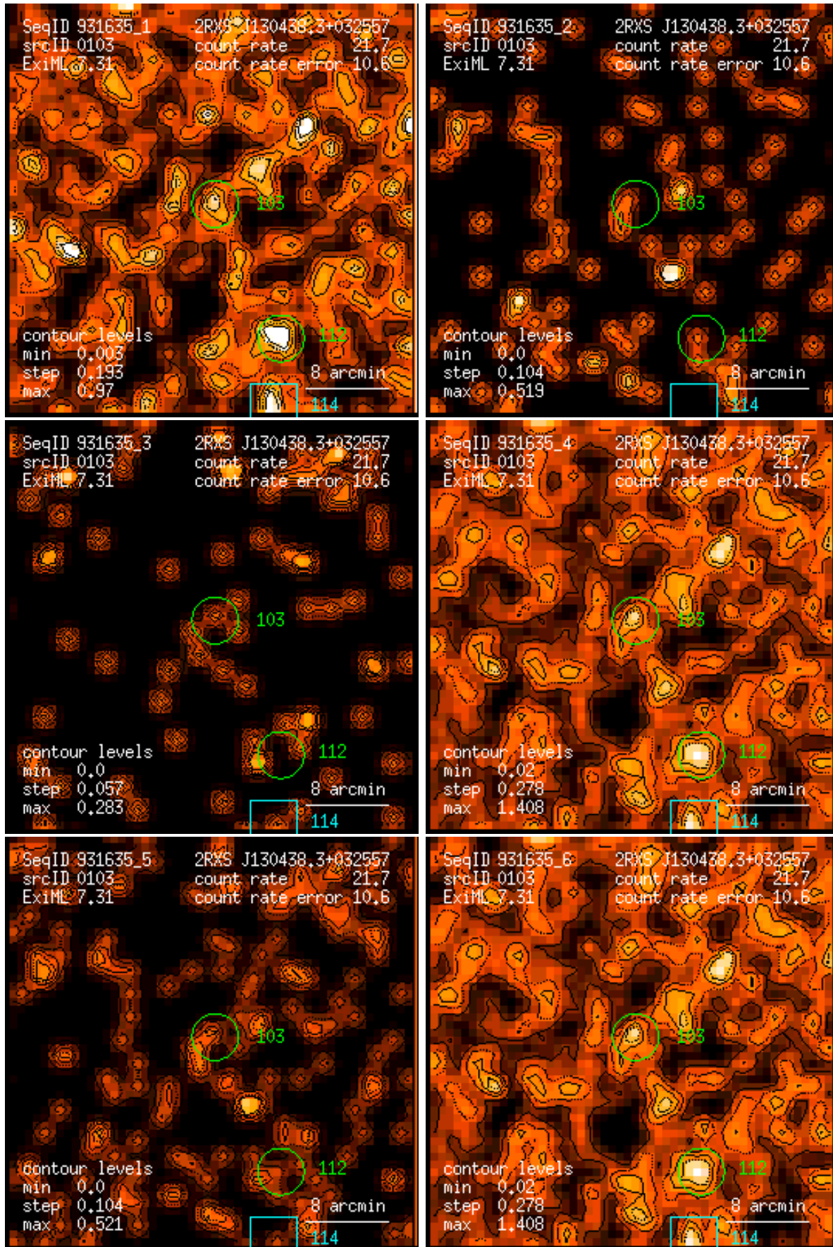
Figure 103: RASS 931635: detection 0103: band rate images, Gaussian filter: (1) PSPC channels 11 – 41, (2) 52 – 90, (3) 91 – 201, (4) 11 – 235, (5) 52 – 201, (6) 11 – 201. Broad band rates in counts/ks. Band rate contour levels in counts/ks/arcmin 2 .
