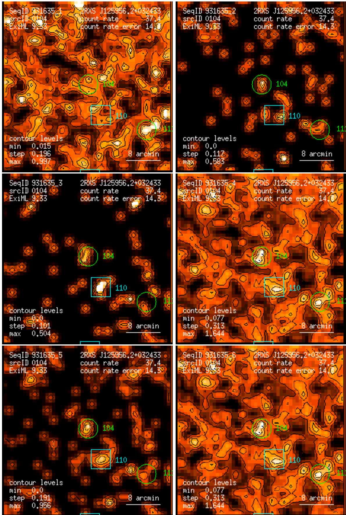
Figure 104: RASS 931635: detection 0104: band rate images, Gaussian filter: (1) PSPC channels 11 – 41, (2) 52 – 90, (3) 91 – 201, (4) 11 – 235, (5) 52 – 201, (6) 11 – 201. Broad band rates in counts/ks. Band rate contour levels in counts/ks/arcmin 2 .
