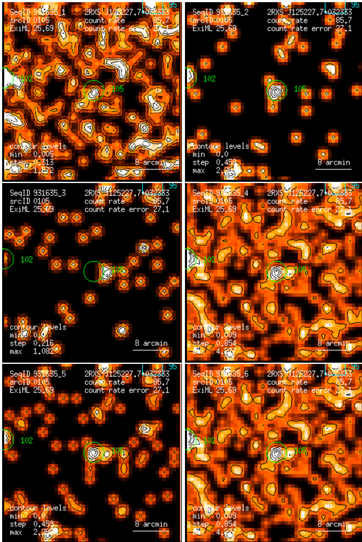
Figure 105: RASS 931635: detection 0105: band rate images, Gaussian filter: (1) PSPC channels 11 – 41, (2) 52 – 90, (3) 91 – 201, (4) 11 – 235, (5) 52 – 201, (6) 11 – 201. Broad band rates in counts/ks. Band rate contour levels in counts/ks/arcmin 2 .
