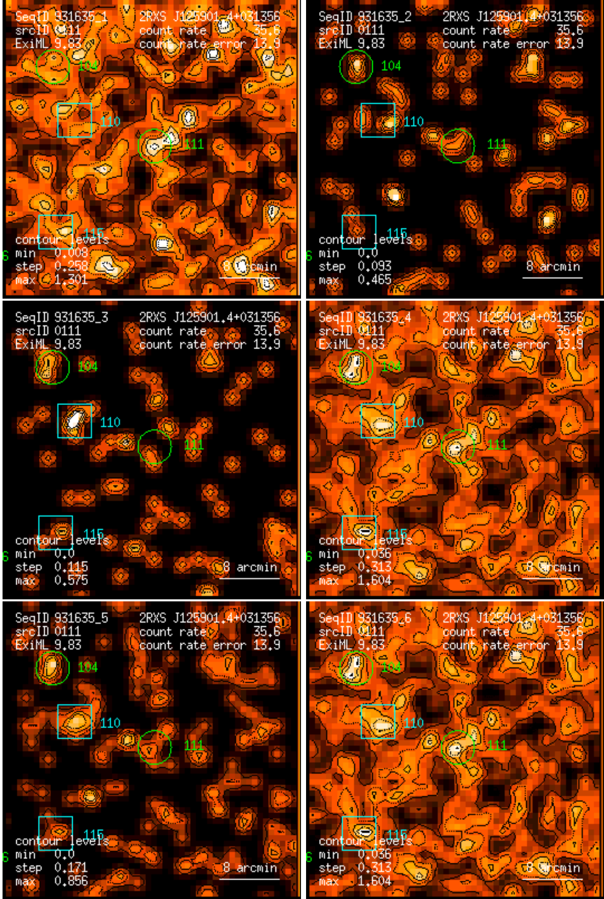
Figure 111: RASS 931635: detection 0111: band rate images, Gaussian filter: (1) PSPC channels 11 – 41, (2) 52 – 90, (3) 91 – 201, (4) 11 – 235, (5) 52 – 201, (6) 11 – 201. Broad band rates in counts/ks. Band rate contour levels in counts/ks/arcmin 2 .
