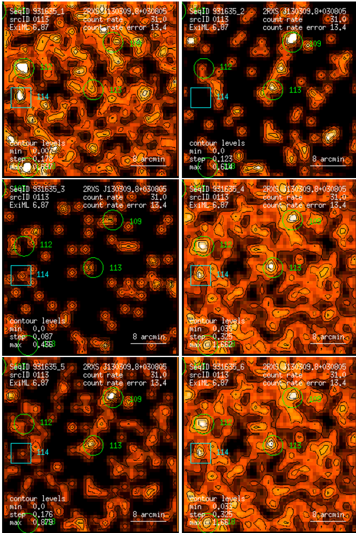
Figure 113: RASS 931635: detection 0113: band rate images, Gaussian filter: (1) PSPC channels 11 – 41, (2) 52 – 90, (3) 91 – 201, (4) 11 – 235, (5) 52 – 201, (6) 11 – 201. Broad band rates in counts/ks. Band rate contour levels in counts/ks/arcmin 2 .
