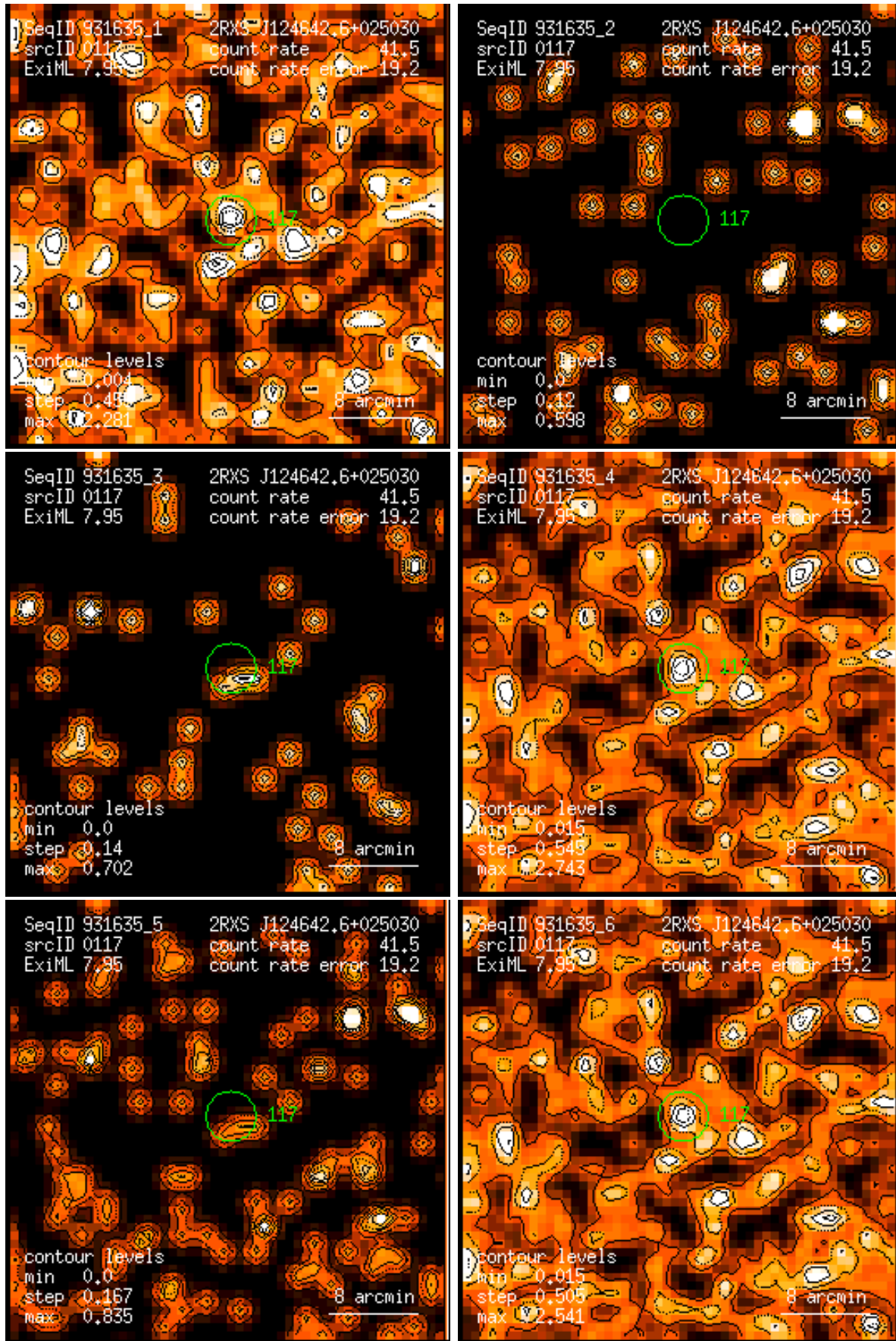
Figure 117: RASS 931635: detection 0117: band rate images, Gaussian filter: (1) PSPC channels 11 – 41, (2) 52 – 90, (3) 91 – 201, (4) 11 – 235, (5) 52 – 201, (6) 11 – 201. Broad band rates in counts/ks. Band rate contour levels in counts/ks/arcmin 2 .
