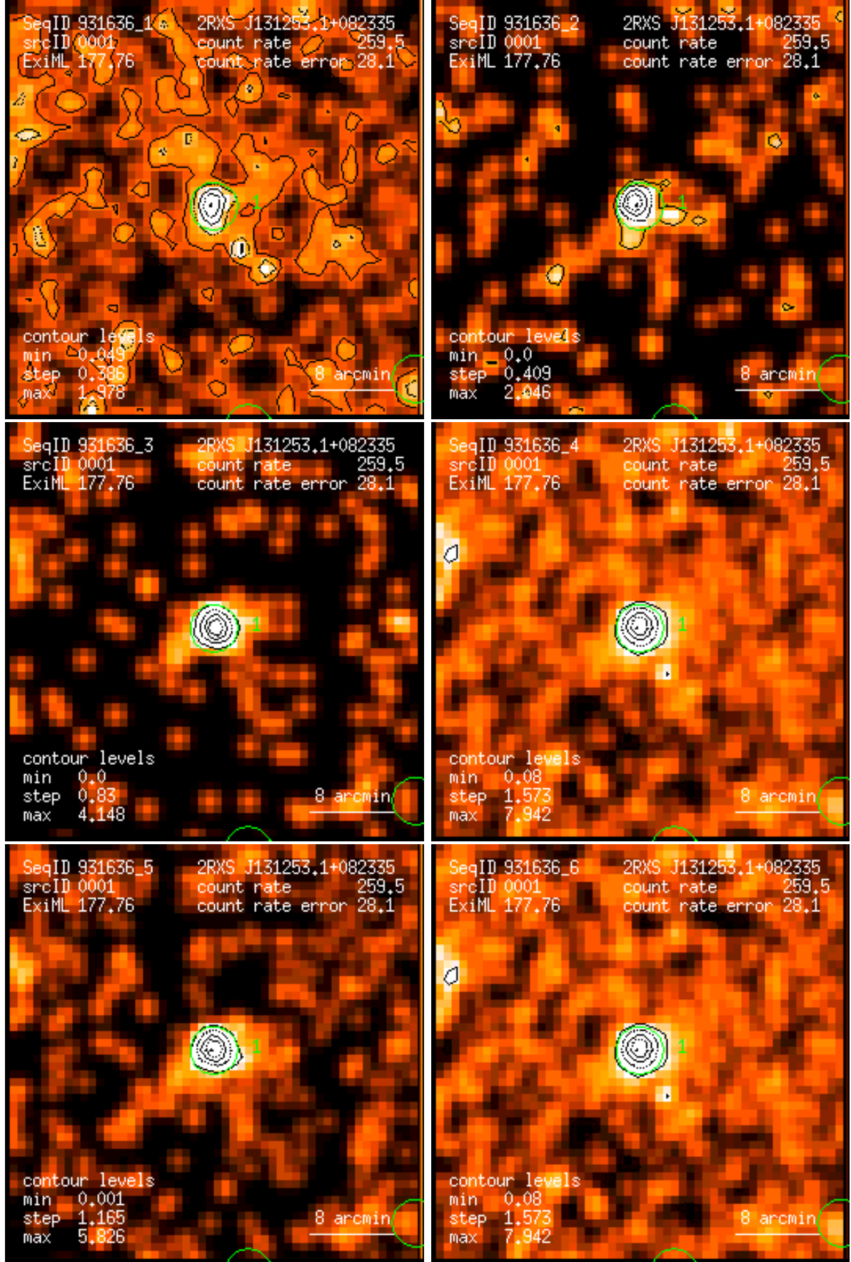
Figure 1: RASS 931636: detection 0001: band rate images, Gaussian filter: (1) PSPC channels 11 – 41, (2) 52 – 90, (3) 91 – 201, (4) 11 – 235, (5) 52 – 201, (6) 11 – 201. Broad band rates in counts/ks. Band rate contour levels in counts/ks/arcmin 2 .
