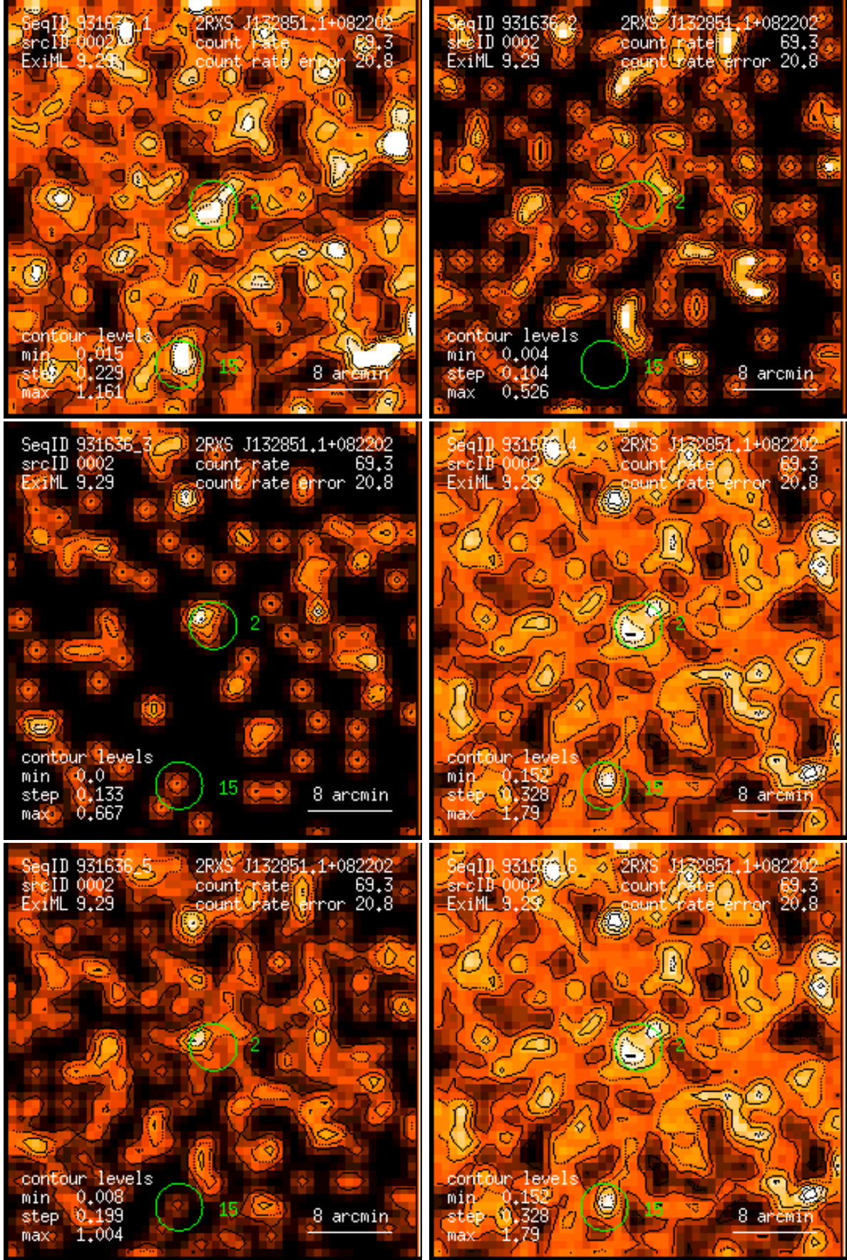
Figure 2: RASS 931636: detection 0002: band rate images, Gaussian filter: (1) PSPC channels 11 – 41, (2) 52 – 90, (3) 91 – 201, (4) 11 – 235, (5) 52 – 201, (6) 11 – 201. Broad band rates in counts/ks. Band rate contour levels in counts/ks/arcmin 2 .
