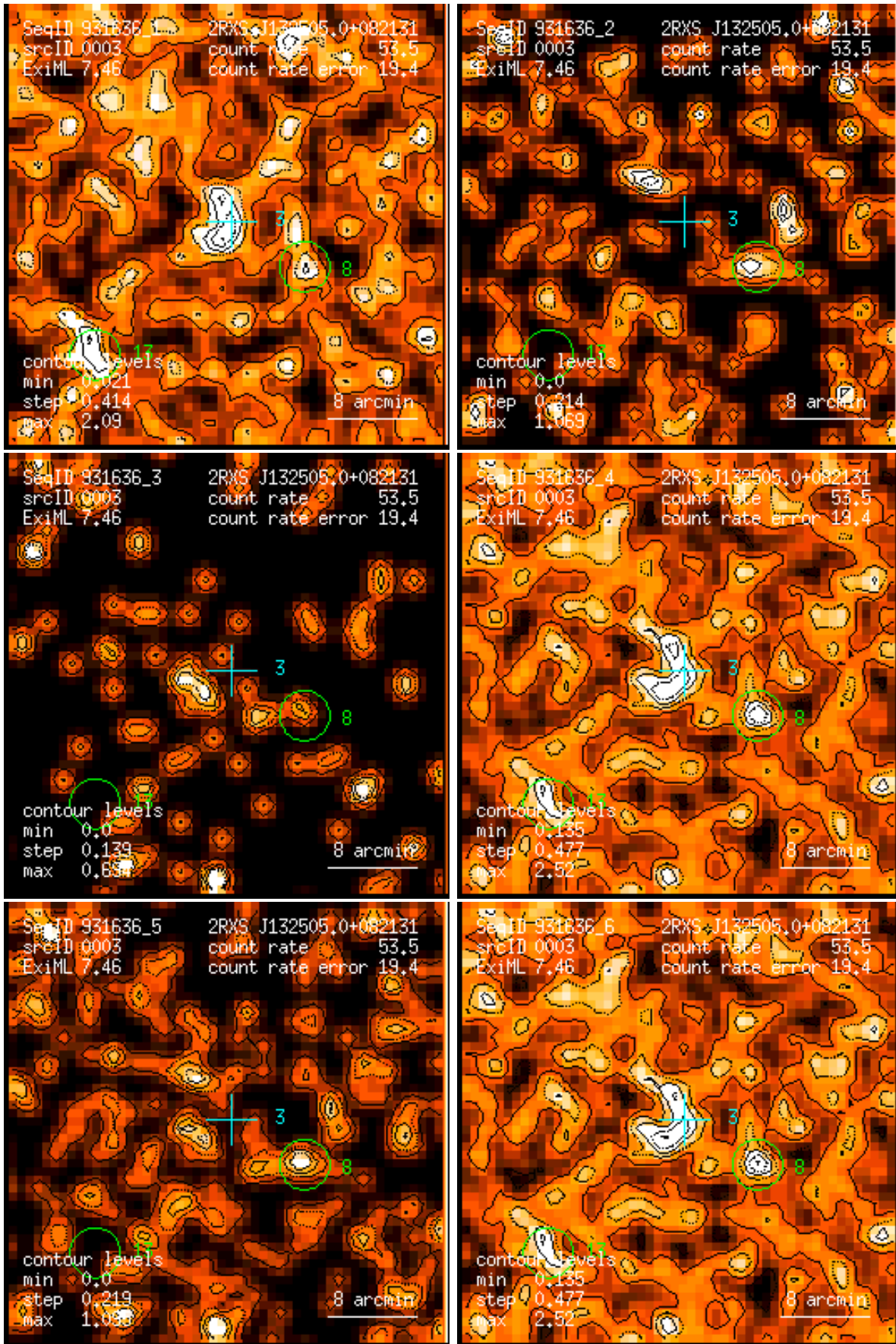
Figure 3: RASS 931636: detection 0003: band rate images, Gaussian filter: (1) PSPC channels 11 – 41, (2) 52 – 90, (3) 91 – 201, (4) 11 – 235, (5) 52 – 201, (6) 11 – 201. Broad band rates in counts/ks. Band rate contour levels in counts/ks/arcmin 2 .
