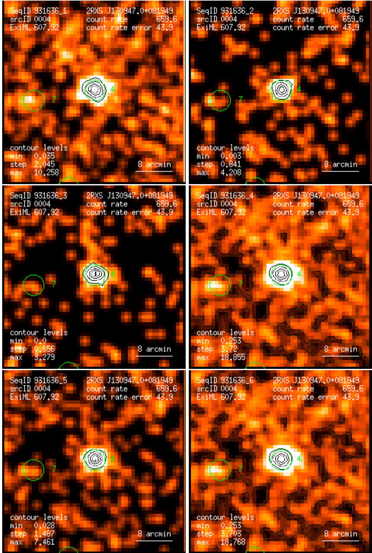
Figure 4: RASS 931636: detection 0004: band rate images, Gaussian filter: (1) PSPC channels 11 – 41, (2) 52 – 90, (3) 91 – 201, (4) 11 – 235, (5) 52 – 201, (6) 11 – 201. Broad band rates in counts/ks. Band rate contour levels in counts/ks/arcmin 2 .
