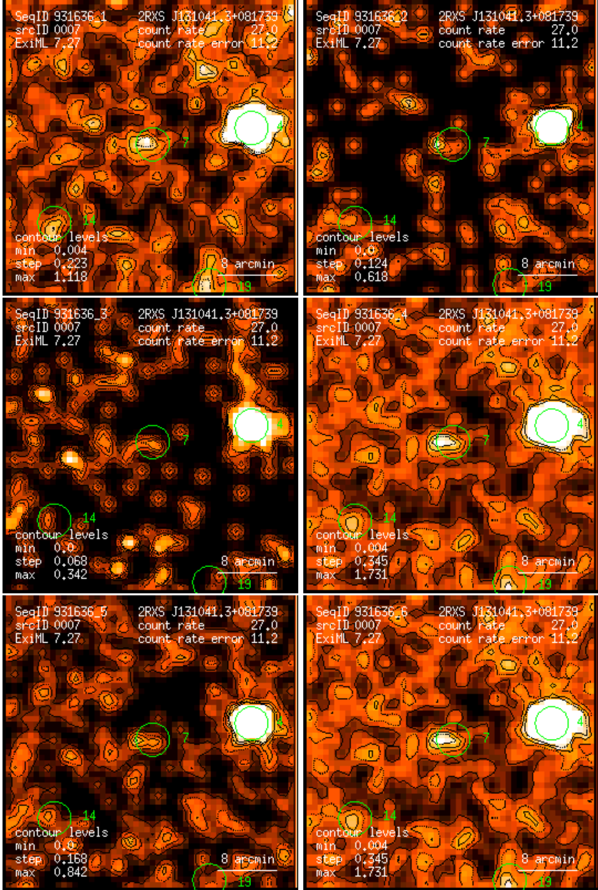
Figure 7: RASS 931636: detection 0007: band rate images, Gaussian filter: (1) PSPC channels 11 – 41, (2) 52 – 90, (3) 91 – 201, (4) 11 – 235, (5) 52 – 201, (6) 11 – 201. Broad band rates in counts/ks. Band rate contour levels in counts/ks/arcmin 2 .
