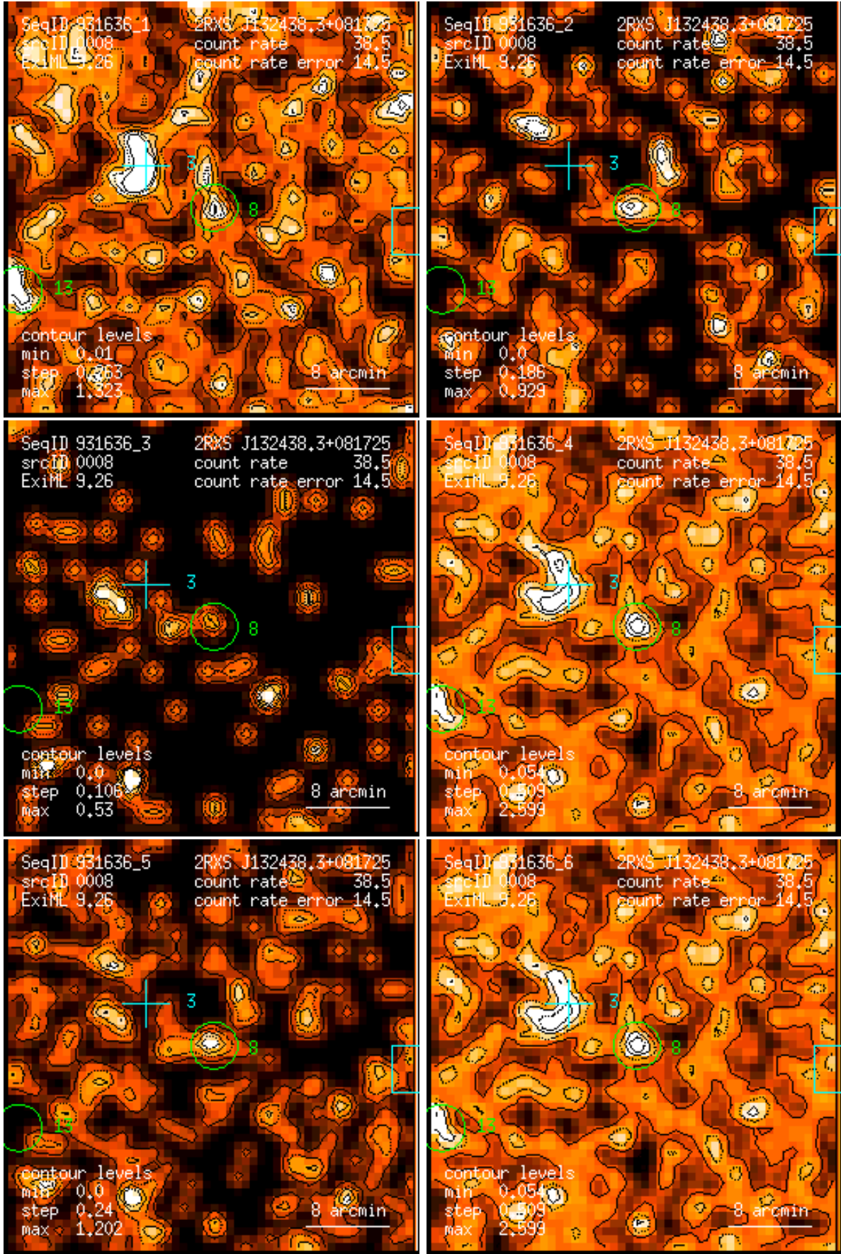
Figure 8: RASS 931636: detection 0008: band rate images, Gaussian filter: (1) PSPC channels 11 – 41, (2) 52 – 90, (3) 91 – 201, (4) 11 – 235, (5) 52 – 201, (6) 11 – 201. Broad band rates in counts/ks. Band rate contour levels in counts/ks/arcmin 2 .
