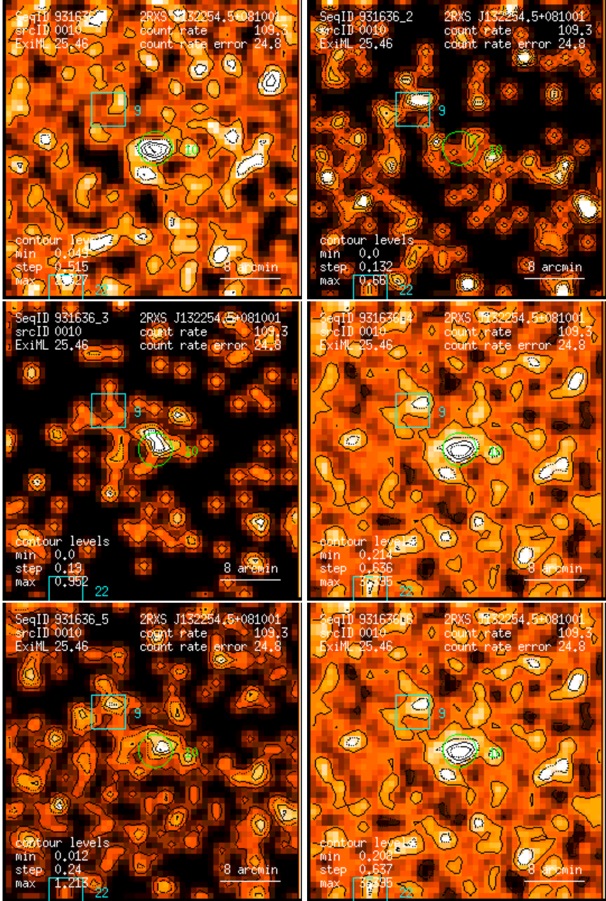
Figure 10: RASS 931636: detection 0010: band rate images, Gaussian filter: (1) PSPC channels 11 – 41, (2) 52 – 90, (3) 91 – 201, (4) 11 – 235, (5) 52 – 201, (6) 11 – 201. Broad band rates in counts/ks. Band rate contour levels in counts/ks/arcmin 2 .
