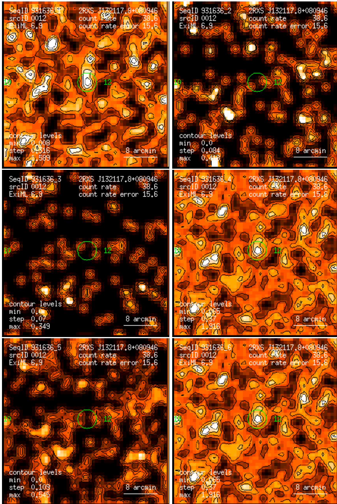
Figure 12: RASS 931636: detection 0012: band rate images, Gaussian filter: (1) PSPC channels 11 – 41, (2) 52 – 90, (3) 91 – 201, (4) 11 – 235, (5) 52 – 201, (6) 11 – 201. Broad band rates in counts/ks. Band rate contour levels in counts/ks/arcmin 2 .
