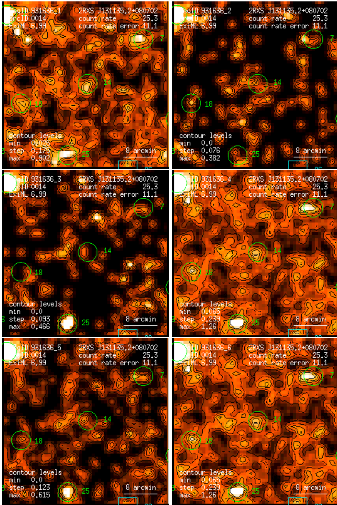
Figure 14: RASS 931636: detection 0014: band rate images, Gaussian filter: (1) PSPC channels 11 – 41, (2) 52 – 90, (3) 91 – 201, (4) 11 – 235, (5) 52 – 201, (6) 11 – 201. Broad band rates in counts/ks. Band rate contour levels in counts/ks/arcmin 2 .
