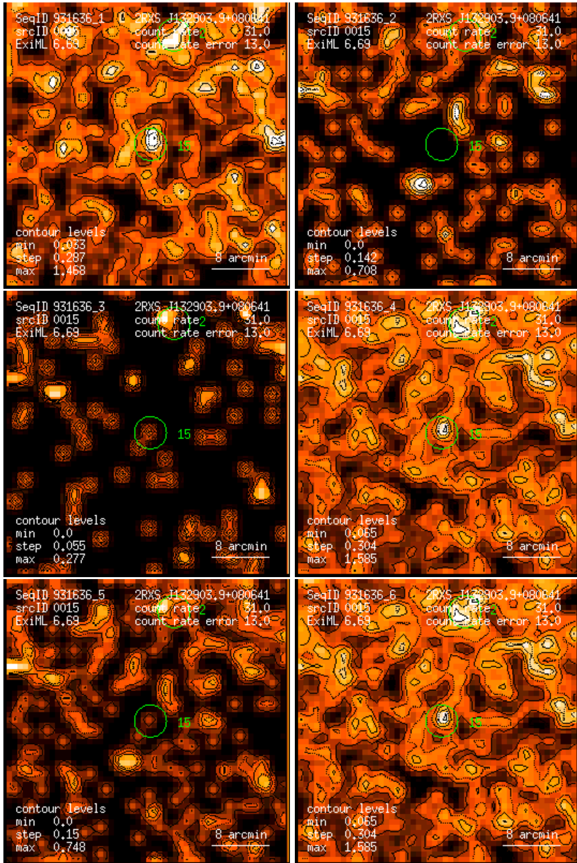
Figure 15: RASS 931636: detection 0015: band rate images, Gaussian filter: (1) PSPC channels 11 – 41, (2) 52 – 90, (3) 91 – 201, (4) 11 – 235, (5) 52 – 201, (6) 11 – 201. Broad band rates in counts/ks. Band rate contour levels in counts/ks/arcmin 2 .
