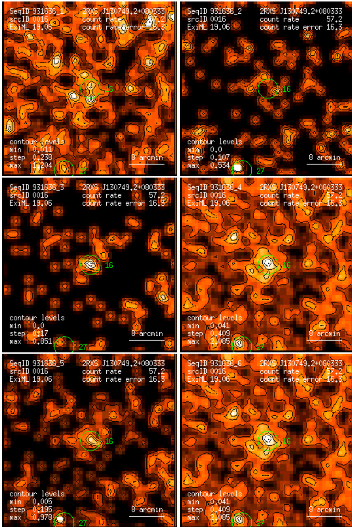
Figure 16: RASS 931636: detection 0016: band rate images, Gaussian filter: (1) PSPC channels 11 – 41, (2) 52 – 90, (3) 91 – 201, (4) 11 – 235, (5) 52 – 201, (6) 11 – 201. Broad band rates in counts/ks. Band rate contour levels in counts/ks/arcmin 2 .
