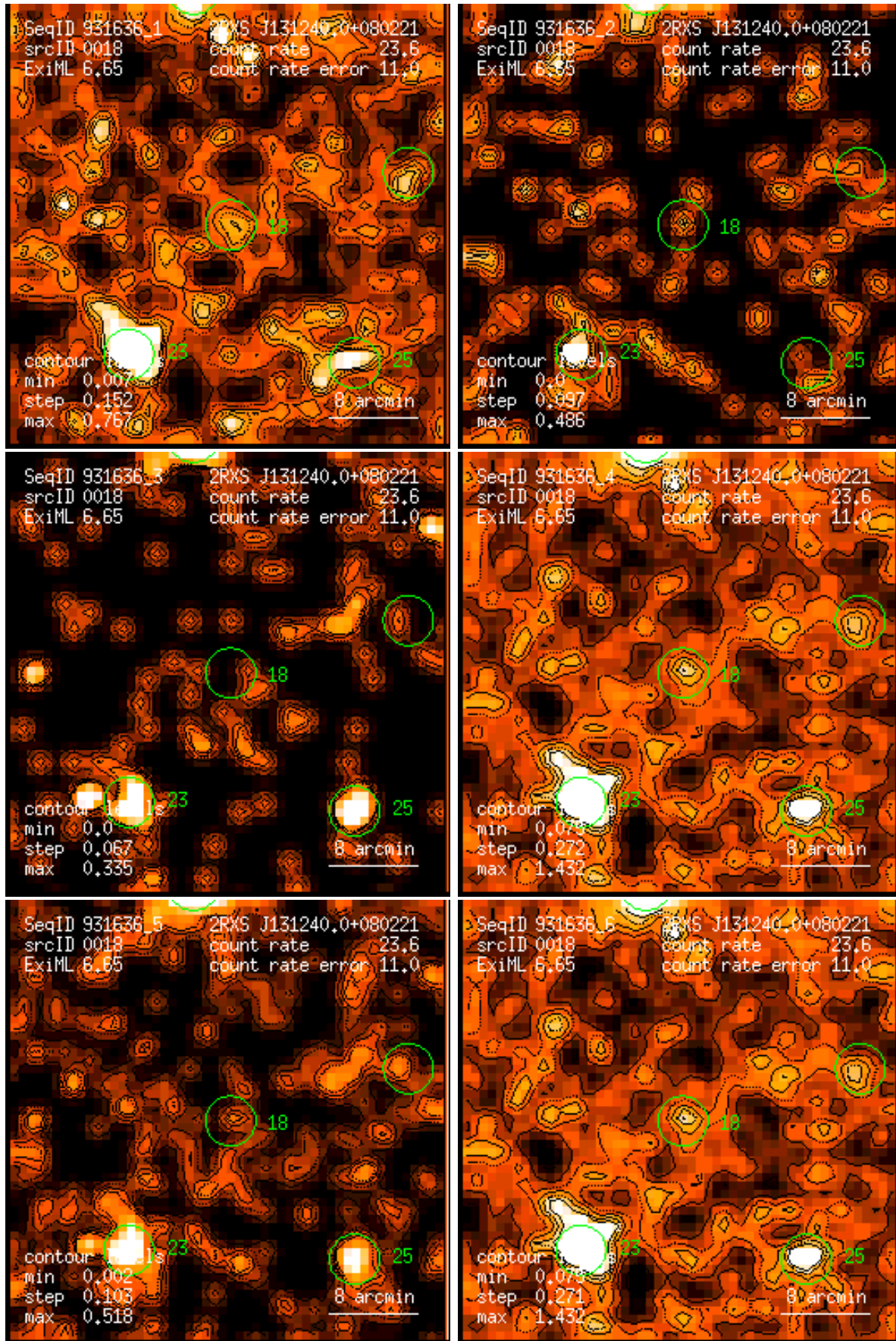
Figure 18: RASS 931636: detection 0018: band rate images, Gaussian filter: (1) PSPC channels 11 – 41, (2) 52 – 90, (3) 91 – 201, (4) 11 – 235, (5) 52 – 201, (6) 11 – 201. Broad band rates in counts/ks. Band rate contour levels in counts/ks/arcmin 2 .
