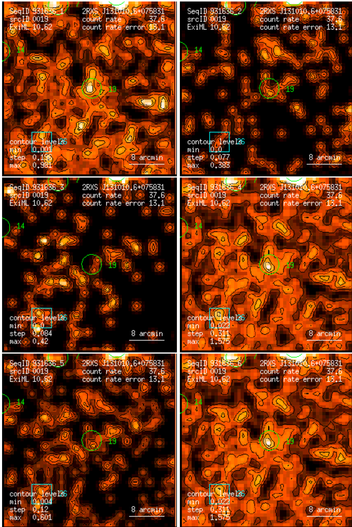
Figure 19: RASS 931636: detection 0019: band rate images, Gaussian filter: (1) PSPC channels 11 – 41, (2) 52 – 90, (3) 91 – 201, (4) 11 – 235, (5) 52 – 201, (6) 11 – 201. Broad band rates in counts/ks. Band rate contour levels in counts/ks/arcmin 2 .
