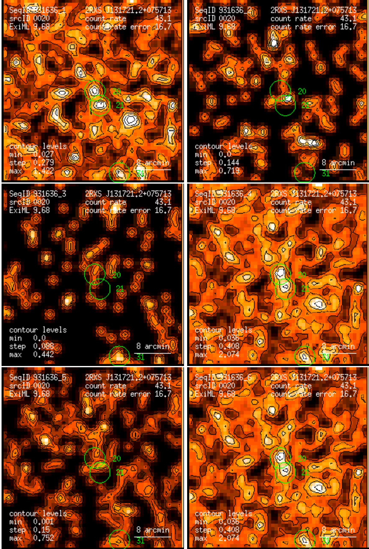
Figure 20: RASS 931636: detection 0020: band rate images, Gaussian filter: (1) PSPC channels 11 – 41, (2) 52 – 90, (3) 91 – 201, (4) 11 – 235, (5) 52 – 201, (6) 11 – 201. Broad band rates in counts/ks. Band rate contour levels in counts/ks/arcmin 2 .
