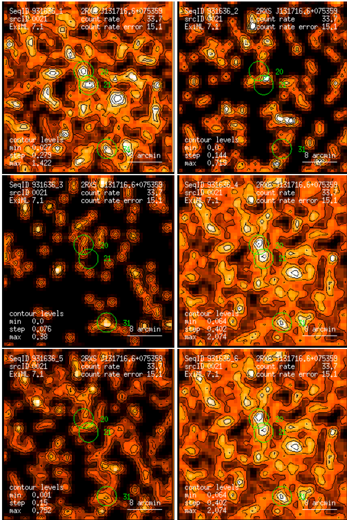
Figure 21: RASS 931636: detection 0021: band rate images, Gaussian filter: (1) PSPC channels 11 – 41, (2) 52 – 90, (3) 91 – 201, (4) 11 – 235, (5) 52 – 201, (6) 11 – 201. Broad band rates in counts/ks. Band rate contour levels in counts/ks/arcmin 2 .
