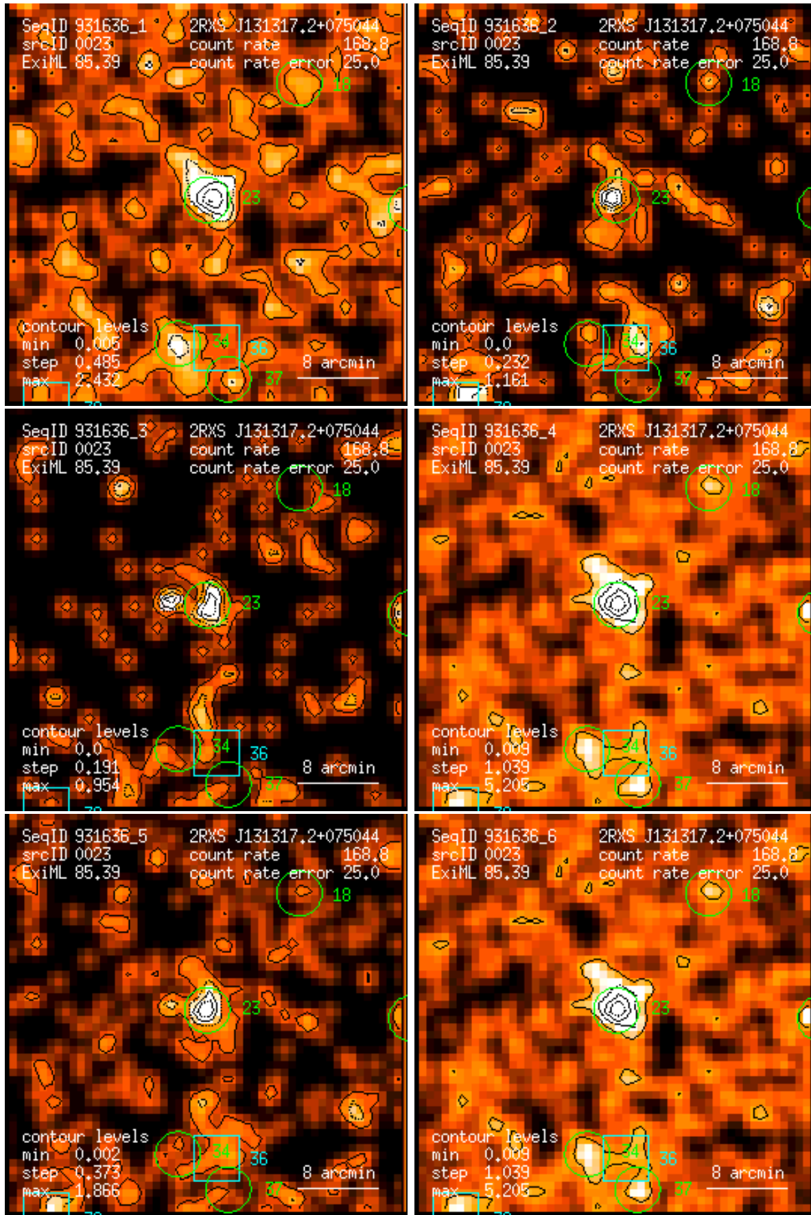
Figure 23: RASS 931636: detection 0023: band rate images, Gaussian filter: (1) PSPC channels 11 – 41, (2) 52 – 90, (3) 91 – 201, (4) 11 – 235, (5) 52 – 201, (6) 11 – 201. Broad band rates in counts/ks. Band rate contour levels in counts/ks/arcmin 2 .
