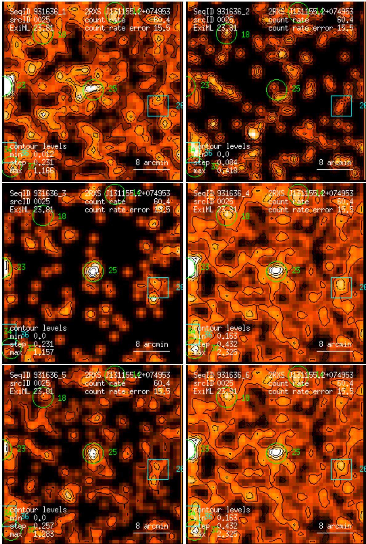
Figure 25: RASS 931636: detection 0025: band rate images, Gaussian filter: (1) PSPC channels 11 – 41, (2) 52 – 90, (3) 91 – 201, (4) 11 – 235, (5) 52 – 201, (6) 11 – 201. Broad band rates in counts/ks. Band rate contour levels in counts/ks/arcmin 2 .
