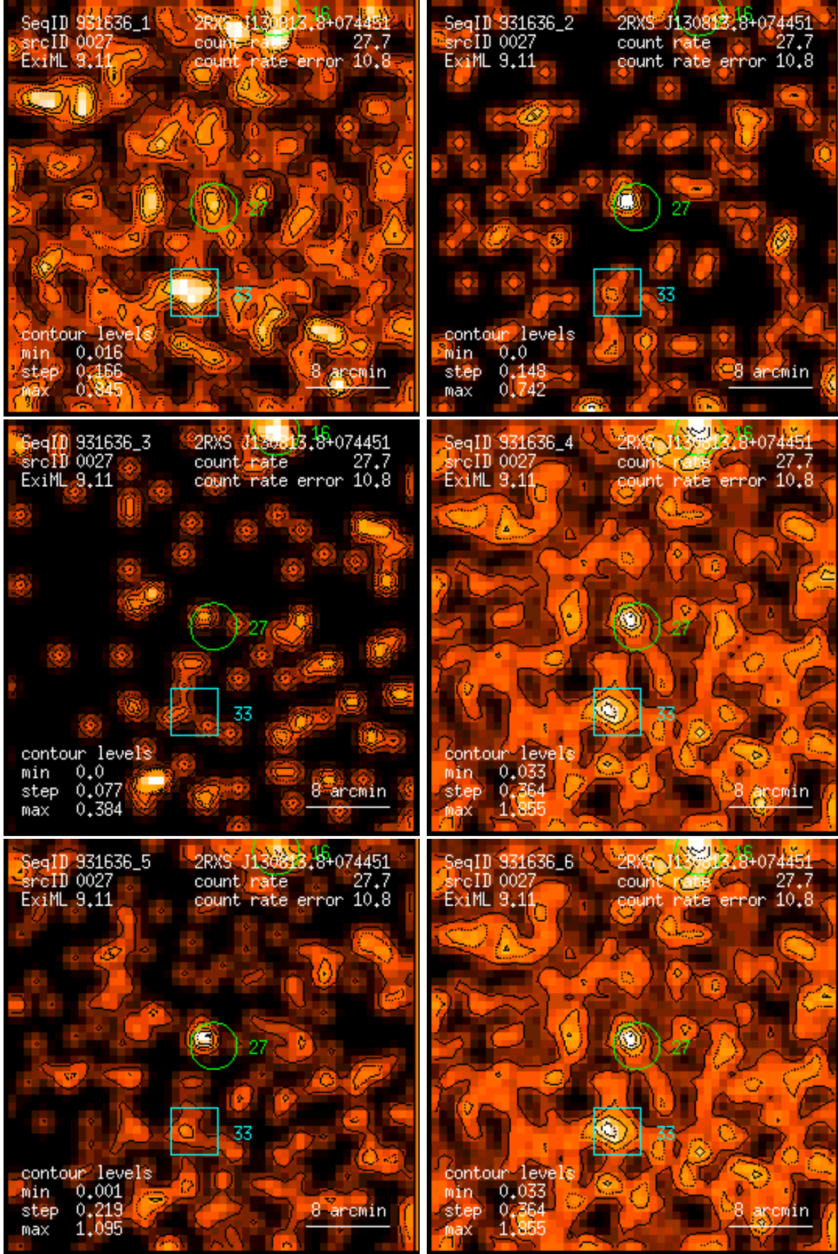
Figure 27: RASS 931636: detection 0027: band rate images, Gaussian filter: (1) PSPC channels 11 – 41, (2) 52 – 90, (3) 91 – 201, (4) 11 – 235, (5) 52 – 201, (6) 11 – 201. Broad band rates in counts/ks. Band rate contour levels in counts/ks/arcmin 2 .
