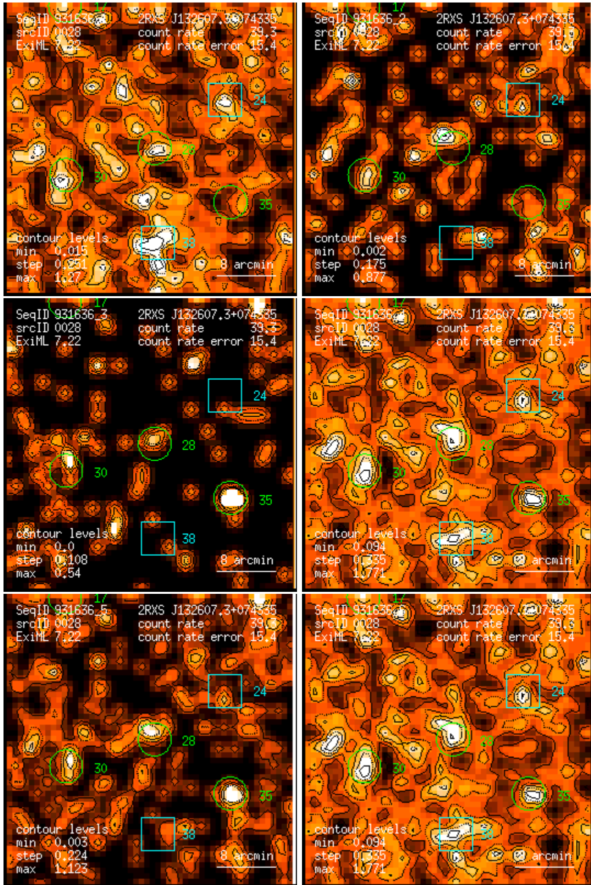
Figure 28: RASS 931636: detection 0028: band rate images, Gaussian filter: (1) PSPC channels 11 – 41, (2) 52 – 90, (3) 91 – 201, (4) 11 – 235, (5) 52 – 201, (6) 11 – 201. Broad band rates in counts/ks. Band rate contour levels in counts/ks/arcmin 2 .
