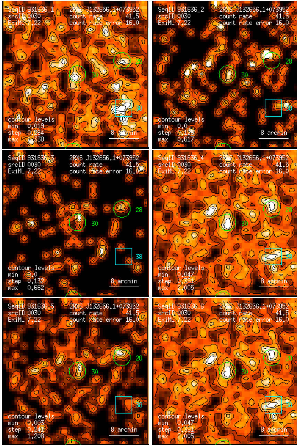
Figure 30: RASS 931636: detection 0030: band rate images, Gaussian filter: (1) PSPC channels 11 – 41, (2) 52 – 90, (3) 91 – 201, (4) 11 – 235, (5) 52 – 201, (6) 11 – 201. Broad band rates in counts/ks. Band rate contour levels in counts/ks/arcmin 2 .
