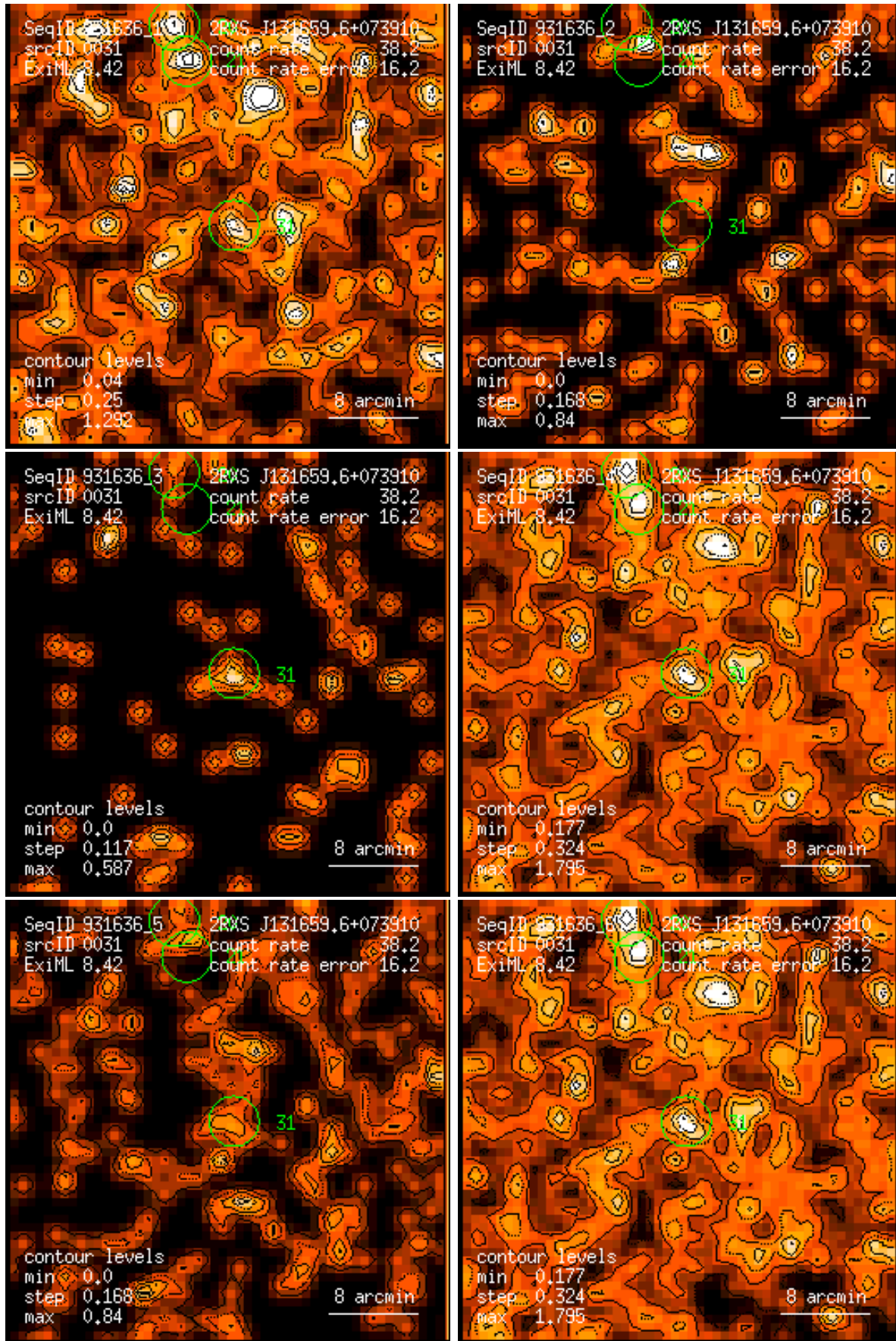
Figure 31: RASS 931636: detection 0031: band rate images, Gaussian filter: (1) PSPC channels 11 – 41, (2) 52 – 90, (3) 91 – 201, (4) 11 – 235, (5) 52 – 201, (6) 11 – 201. Broad band rates in counts/ks. Band rate contour levels in counts/ks/arcmin 2 .
