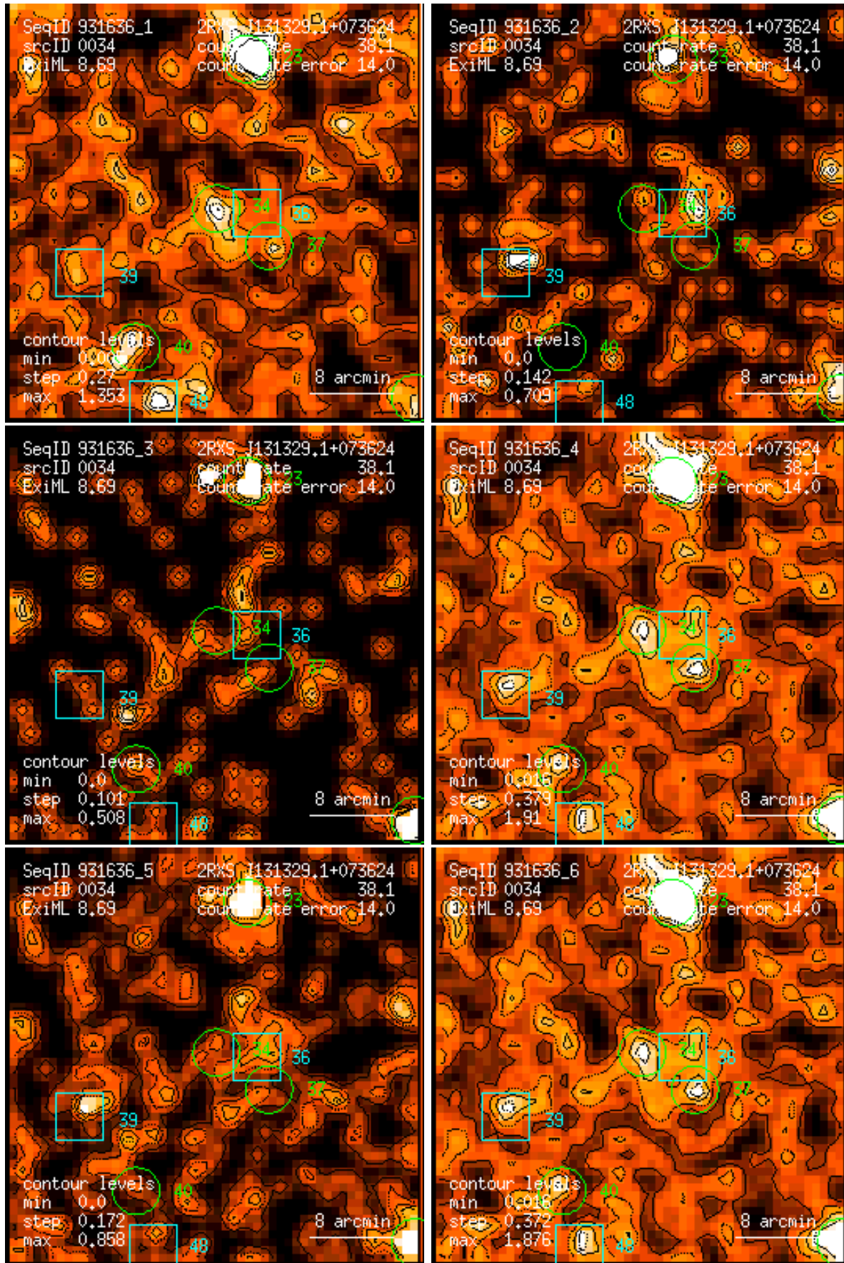
Figure 34: RASS 931636: detection 0034: band rate images, Gaussian filter: (1) PSPC channels 11 – 41, (2) 52 – 90, (3) 91 – 201, (4) 11 – 235, (5) 52 – 201, (6) 11 – 201. Broad band rates in counts/ks. Band rate contour levels in counts/ks/arcmin 2 .
