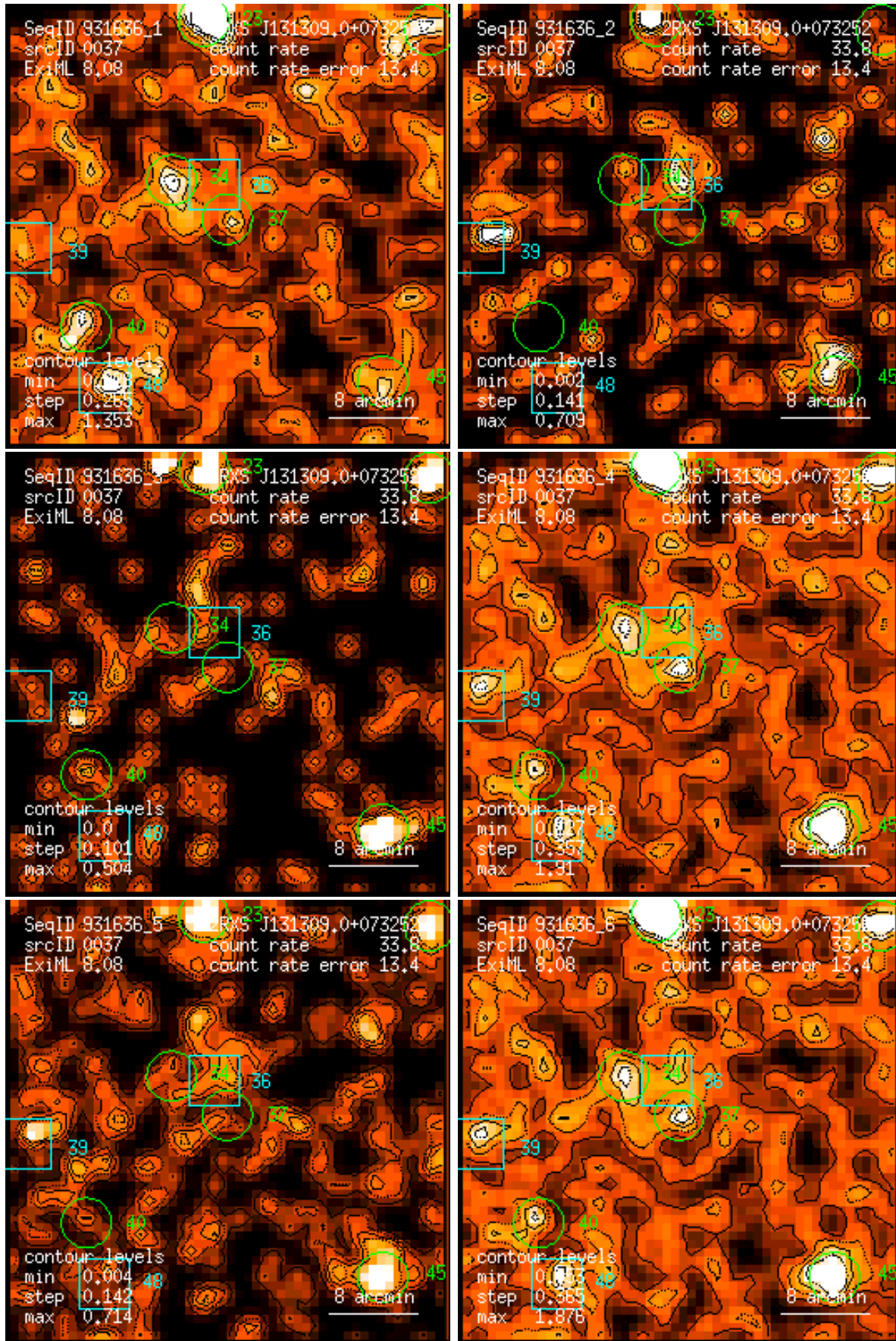
Figure 37: RASS 931636: detection 0037: band rate images, Gaussian filter: (1) PSPC channels 11 – 41, (2) 52 – 90, (3) 91 – 201, (4) 11 – 235, (5) 52 – 201, (6) 11 – 201. Broad band rates in counts/ks. Band rate contour levels in counts/ks/arcmin 2 .
