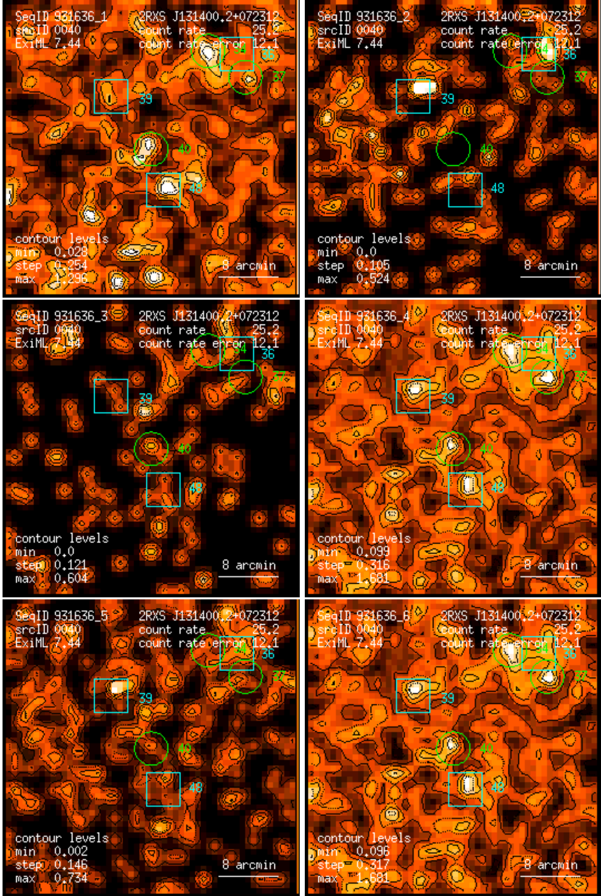
Figure 40: RASS 931636: detection 0040: band rate images, Gaussian filter: (1) PSPC channels 11 – 41, (2) 52 – 90, (3) 91 – 201, (4) 11 – 235, (5) 52 – 201, (6) 11 – 201. Broad band rates in counts/ks. Band rate contour levels in counts/ks/arcmin 2 .
