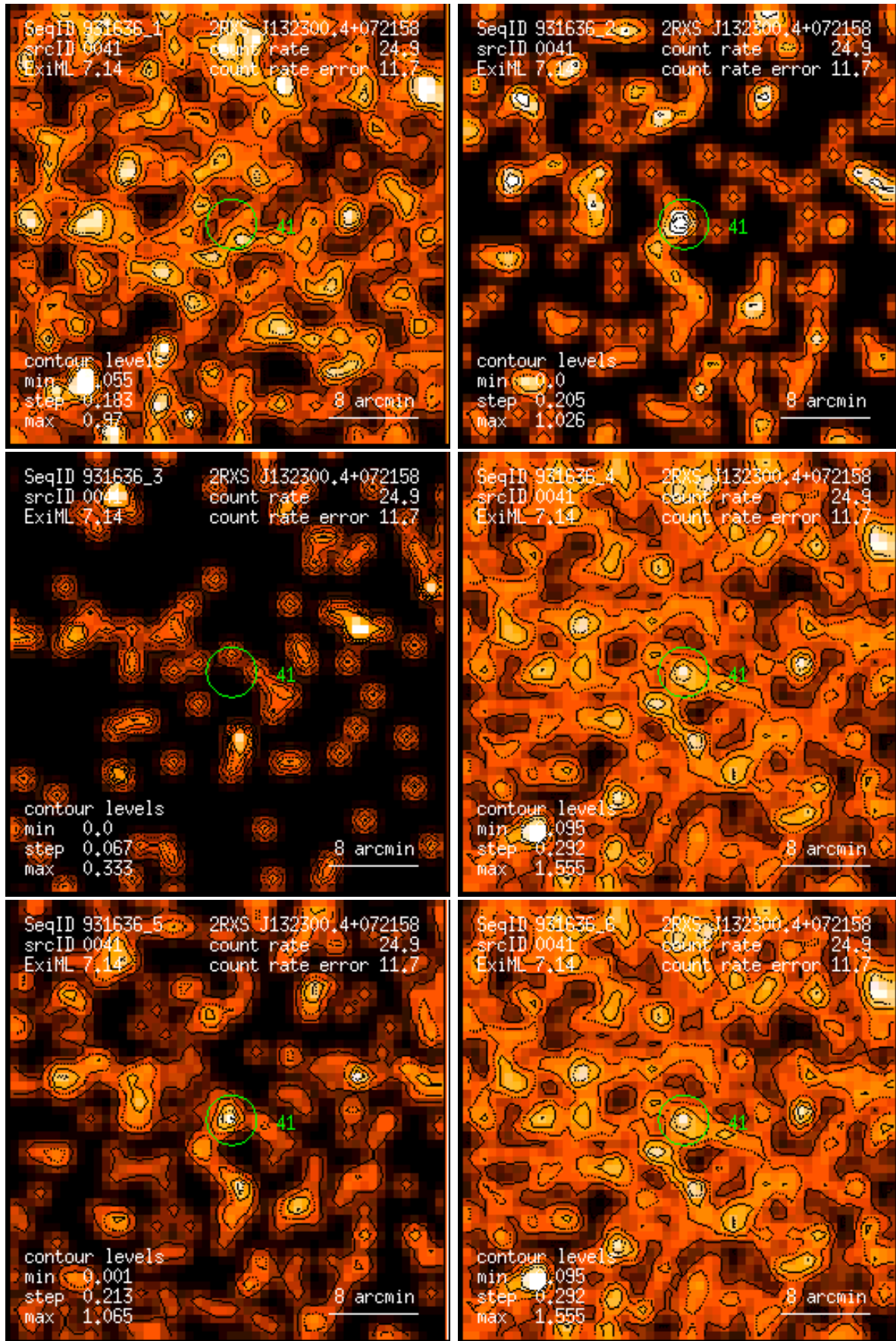
Figure 41: RASS 931636: detection 0041: band rate images, Gaussian filter: (1) PSPC channels 11 – 41, (2) 52 – 90, (3) 91 – 201, (4) 11 – 235, (5) 52 – 201, (6) 11 – 201. Broad band rates in counts/ks. Band rate contour levels in counts/ks/arcmin 2 .
