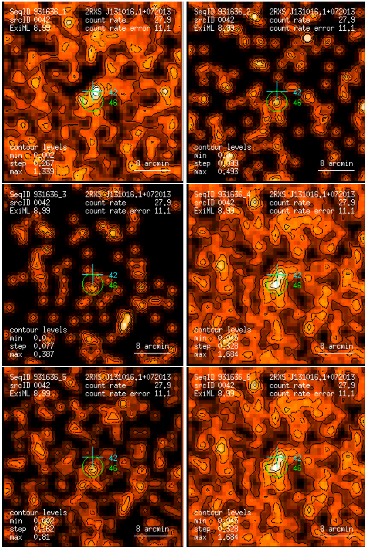
Figure 42: RASS 931636: detection 0042: band rate images, Gaussian filter: (1) PSPC channels 11 – 41, (2) 52 – 90, (3) 91 – 201, (4) 11 – 235, (5) 52 – 201, (6) 11 – 201. Broad band rates in counts/ks. Band rate contour levels in counts/ks/arcmin 2 .
