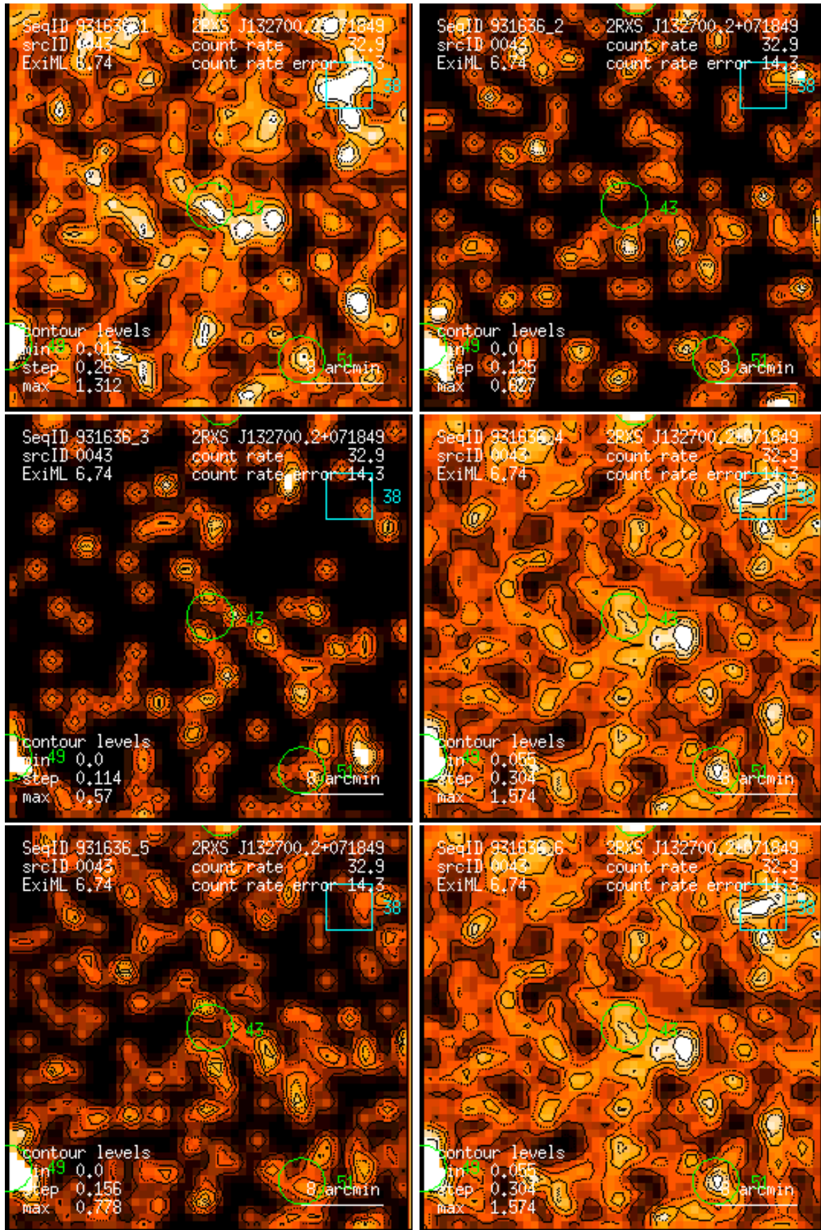
Figure 43: RASS 931636: detection 0043: band rate images, Gaussian filter: (1) PSPC channels 11 – 41, (2) 52 – 90, (3) 91 – 201, (4) 11 – 235, (5) 52 – 201, (6) 11 – 201. Broad band rates in counts/ks. Band rate contour levels in counts/ks/arcmin 2 .
