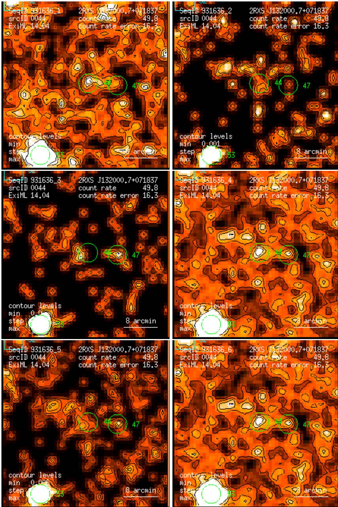
Figure 44: RASS 931636: detection 0044: band rate images, Gaussian filter: (1) PSPC channels 11 – 41, (2) 52 – 90, (3) 91 – 201, (4) 11 – 235, (5) 52 – 201, (6) 11 – 201. Broad band rates in counts/ks. Band rate contour levels in counts/ks/arcmin 2 .
