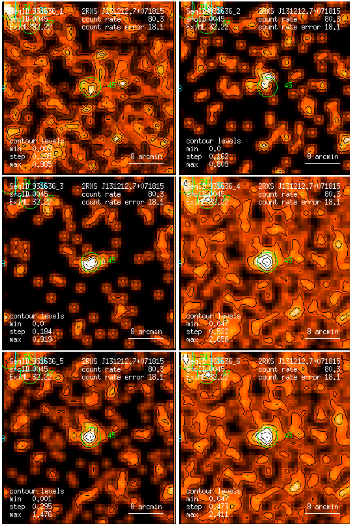
Figure 45: RASS 931636: detection 0045: band rate images, Gaussian filter: (1) PSPC channels 11 – 41, (2) 52 – 90, (3) 91 – 201, (4) 11 – 235, (5) 52 – 201, (6) 11 – 201. Broad band rates in counts/ks. Band rate contour levels in counts/ks/arcmin 2 .
